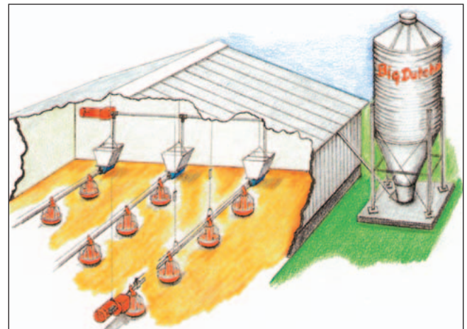
Illustration of a house with AugerMatic lines
