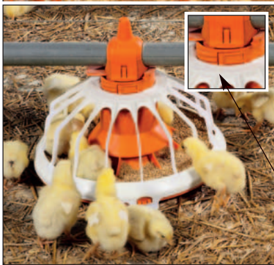
FLUXX 360 with corrugated bottom, feed shut-off and 16-arm grill
