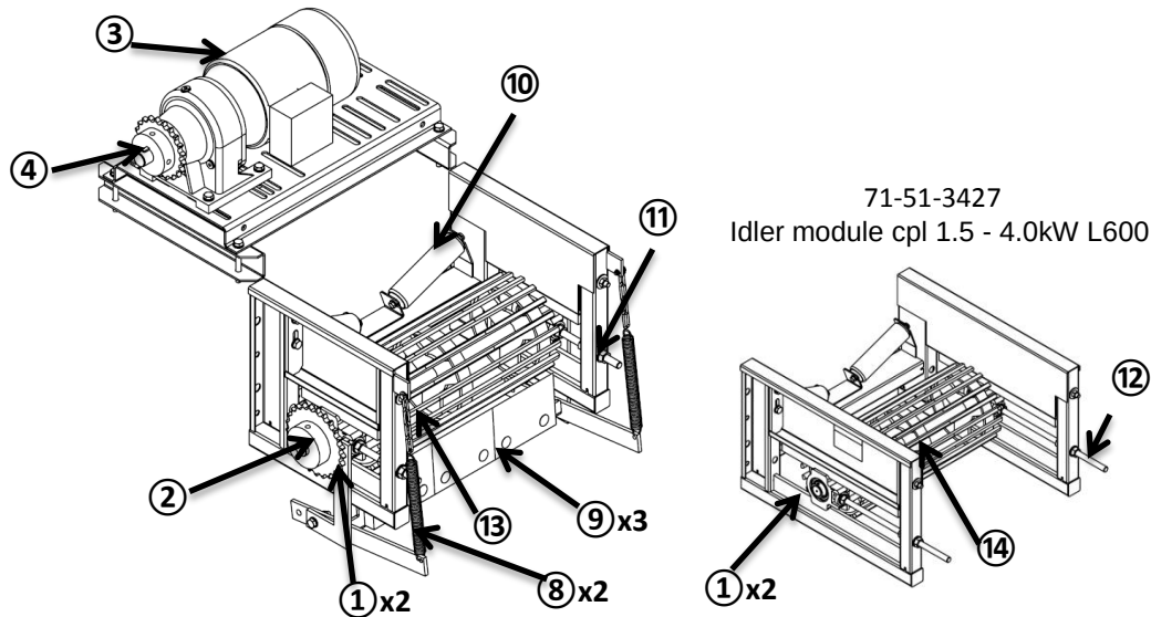
Drive 2.2kW Elevated Conveyor Belt Unit
