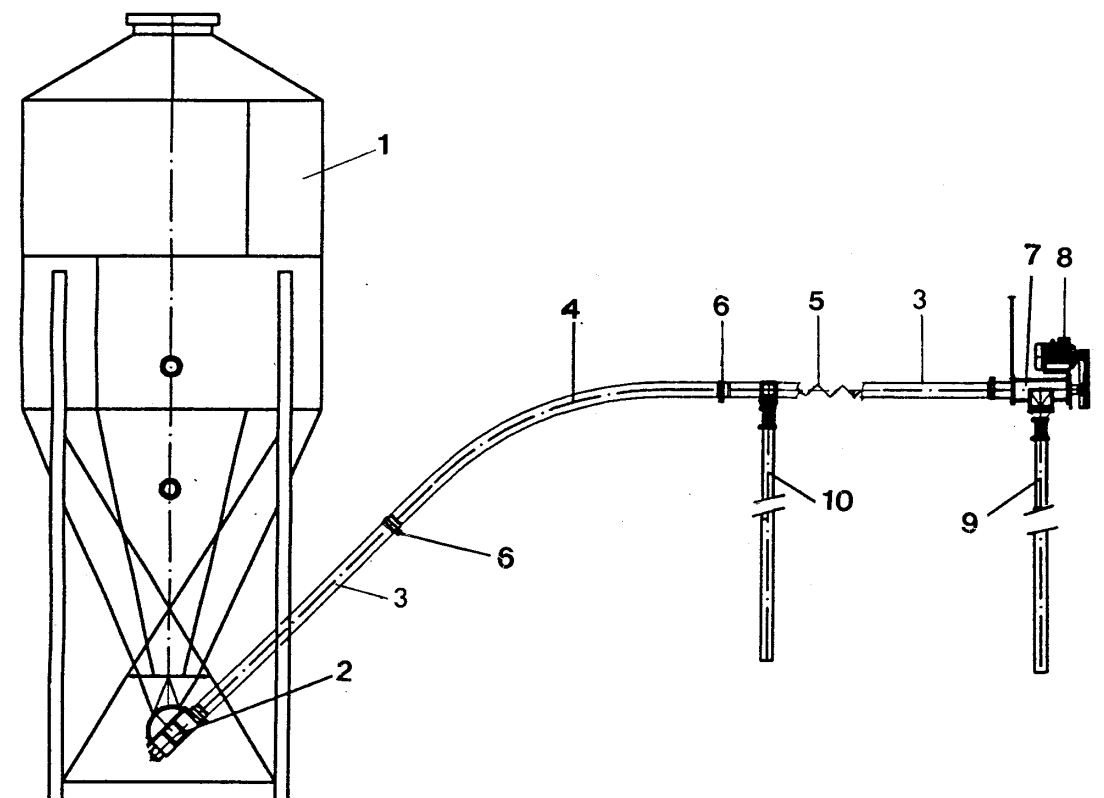
figure 1: Schematic construction of a Flex-Vey.
