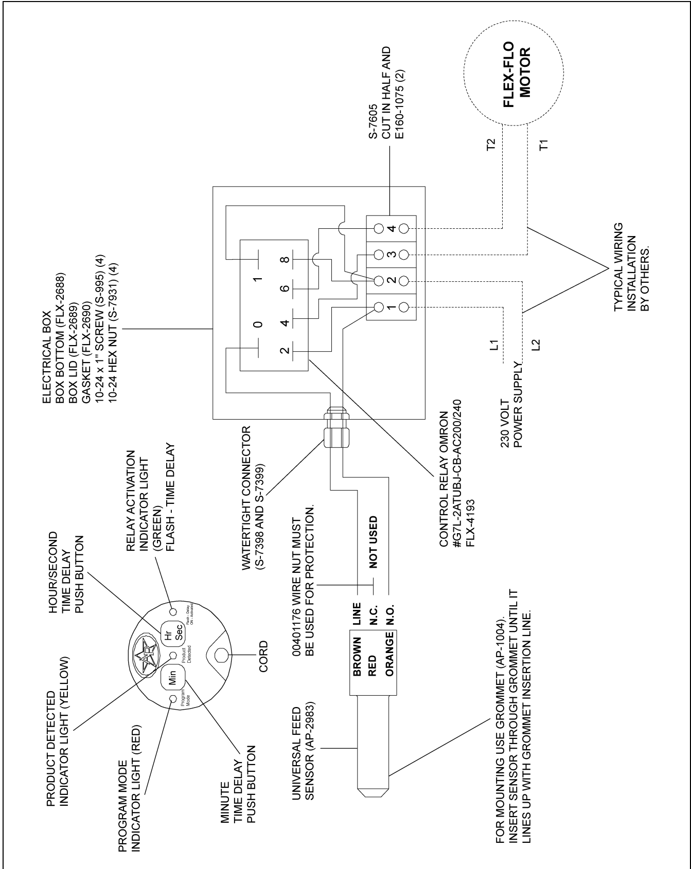
Figure 2 Wiring Diagram for FLX-4246A
